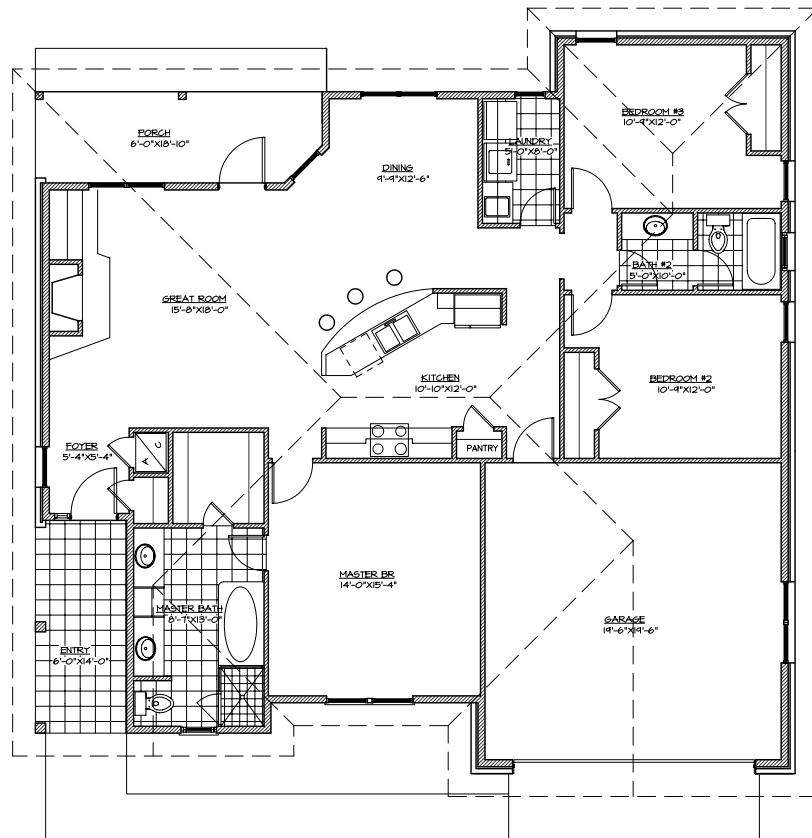
1 FLOOR PLAN * B-1 SCALE: NTS
