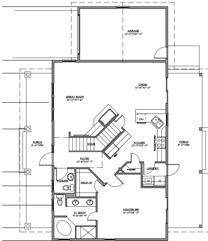
1. 1ST FLOOR PLAN * D-1 SCALE: NTS
