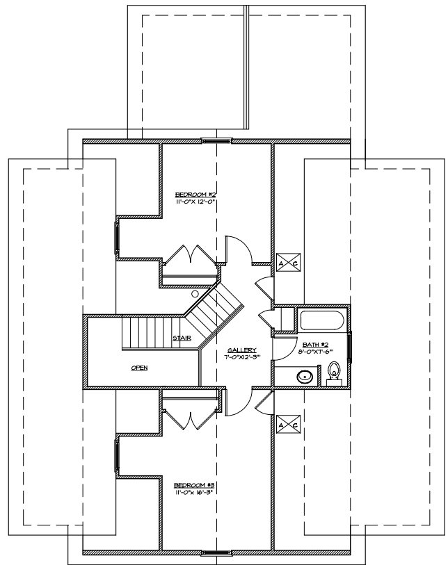
2. 2ND FLOOR PLAN SCALE: NTS
